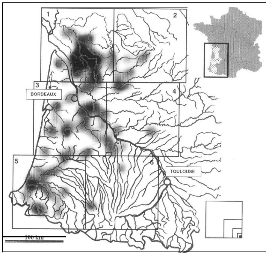
Fig. 1. Gaussian representation of European mink, Mustela lutreola , population in Southwestern France. (Lower right: squares show the 5 reiterated divisions of the 6 main areas for fractal analysis).
