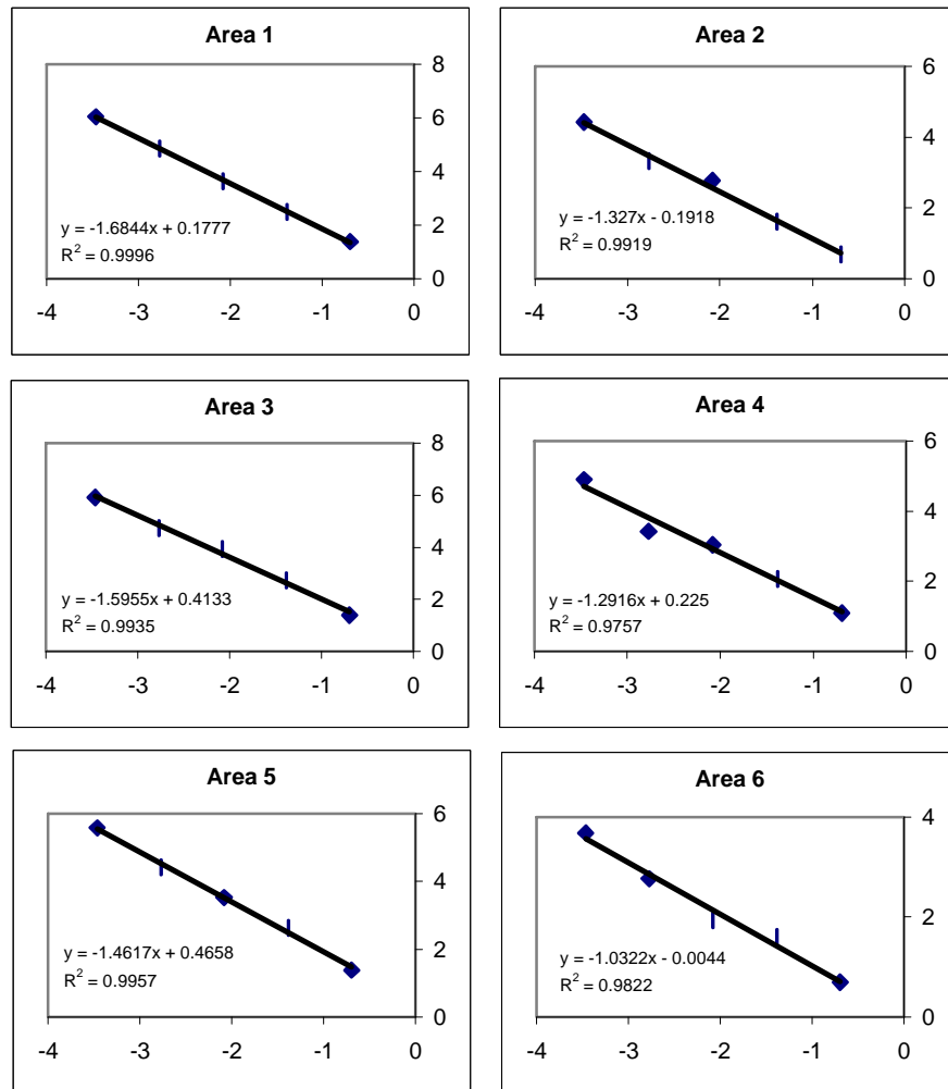
Fig. 2. Ln-In regression analysis considering number of squares where mink were evidenced ( y = \ln number of squares for each iteration) and scale of resolution ( x = \ln resolution for each iteration, as \ln 0.5 , \ln 0.25 , \ln 0.125 , \ln 0.0625 , \ln 0.03125 ) for the 6 areas inhabited by the Mustela lutreola western population (France).
